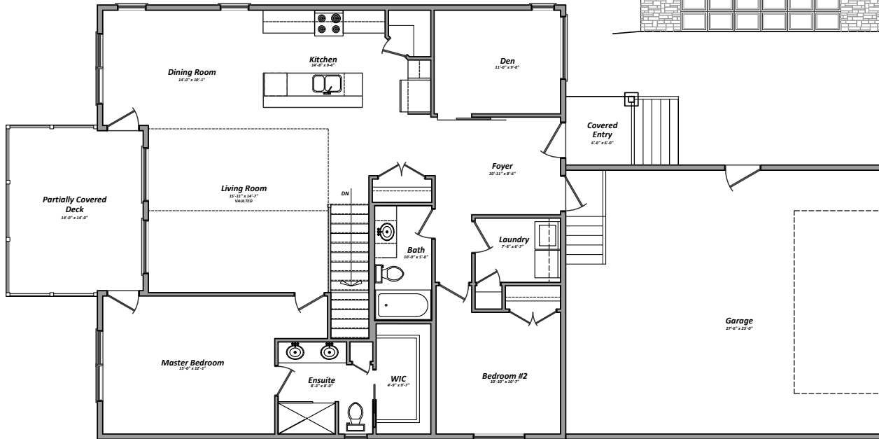
Main Floor Plan 1502 ft 2
