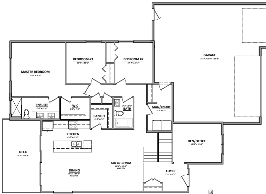
Main Floor Plan 1688 ft2
